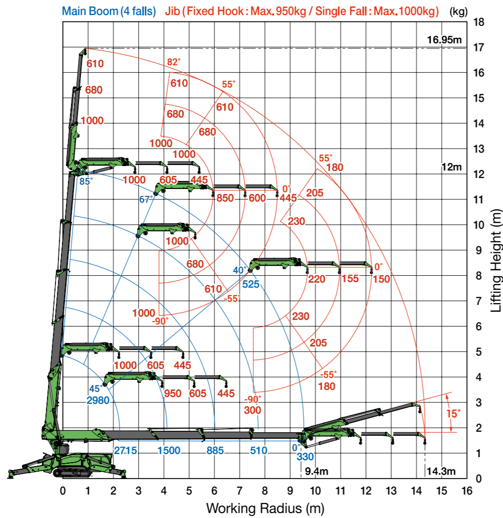
This working range chart shows total rated load including boom deflection.
